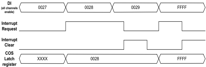
Figure 3-6: COS Example
