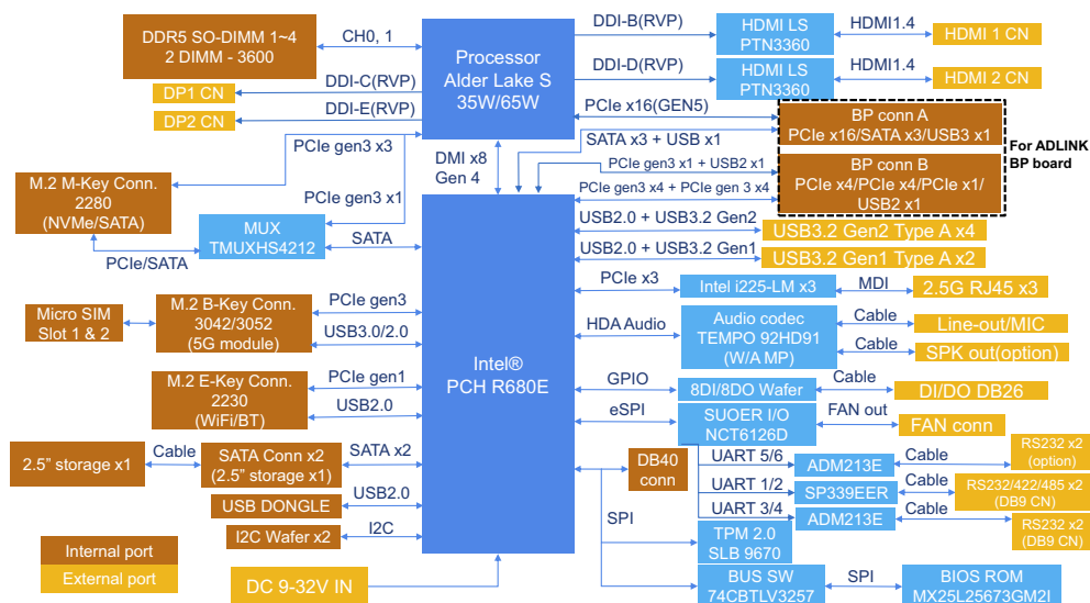
Figure 2-1: MVP-6200 Series Functional Block Diagram
