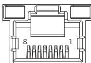
Figure 3-8: Ethernet Port and LEDs
