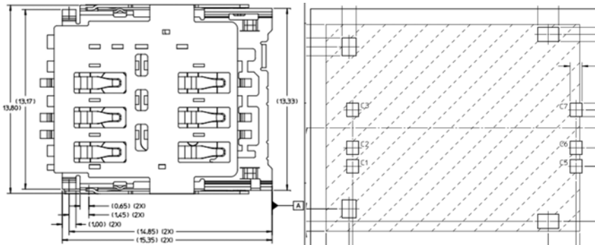
Figure 3-20: Micro-SIM Slot
