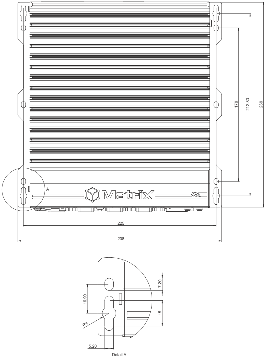
Figure 2-2: MVP-6200 Series Top View
