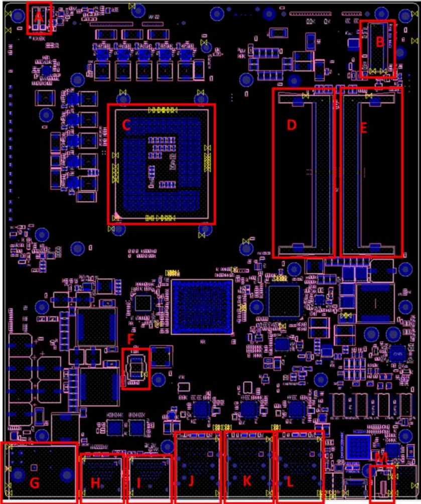
Figure 3-11: Mainboard Top Connectors
