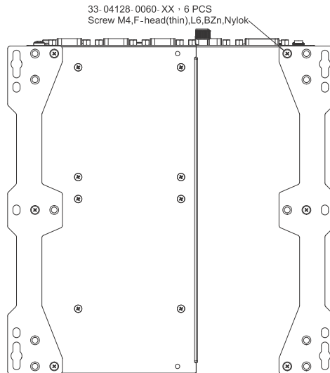
Bottom Panel Mounting Bracket Orientation
