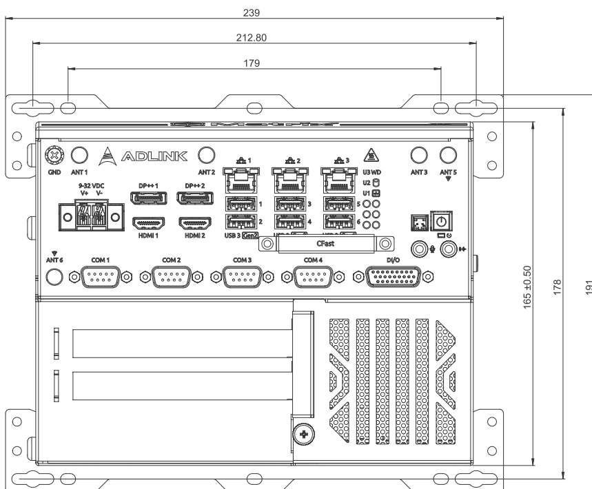
Figure 2-3: MVP-6200 Series 2 Slot Front View
