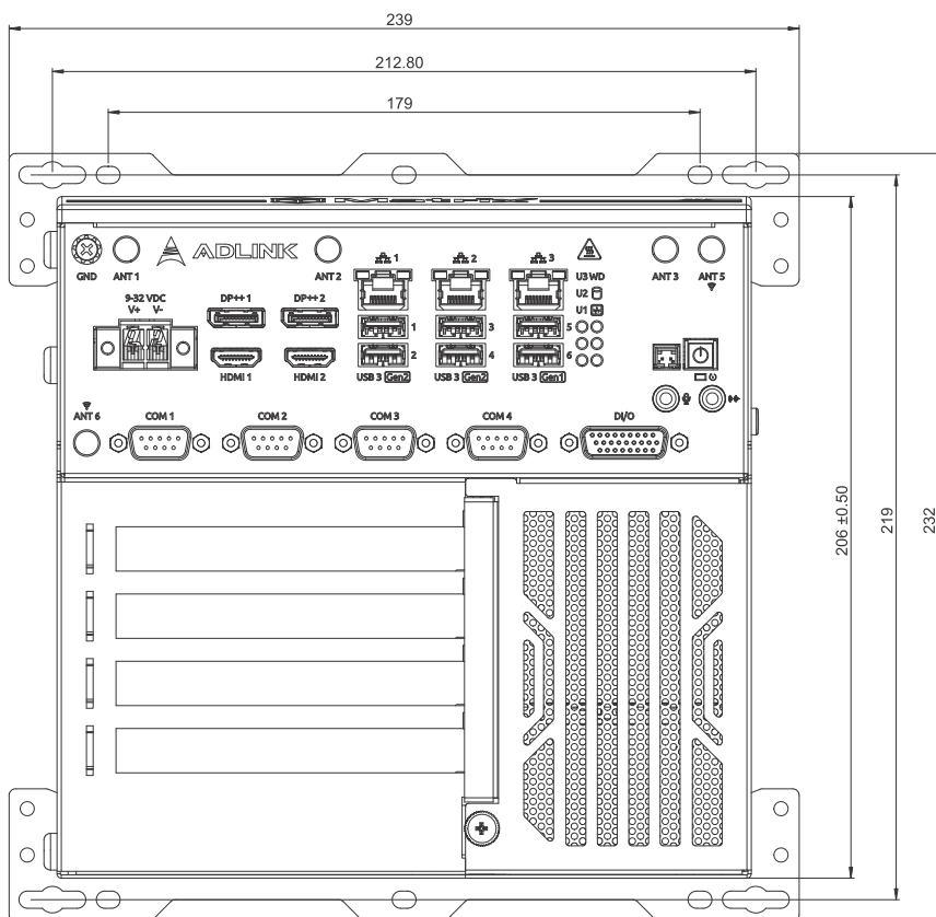
Figure 2-5: MVP-6200 Series 4 Slot Front View
