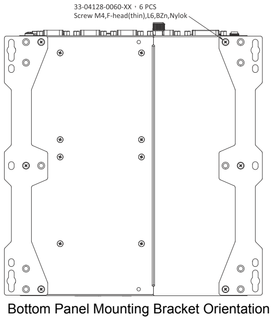
Figure 2-4: MVP-6200 Series 2 Slot Mounting
