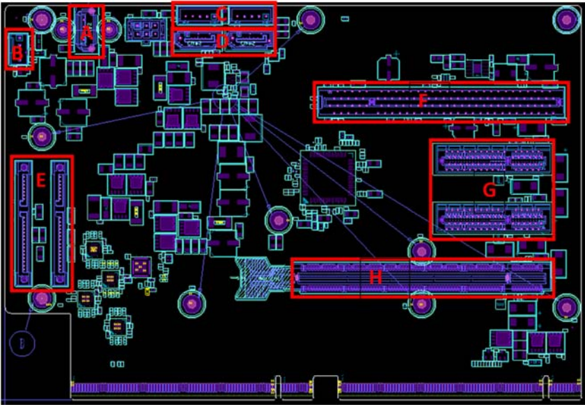
Figure 3-14: 4-slot Backplane Card
