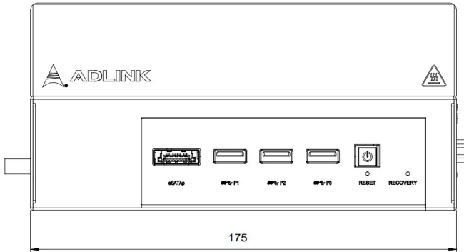
Figure 1-1: Front View Dimensions
