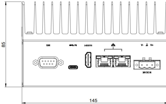
Figure 1-2: Side View Dimensions
