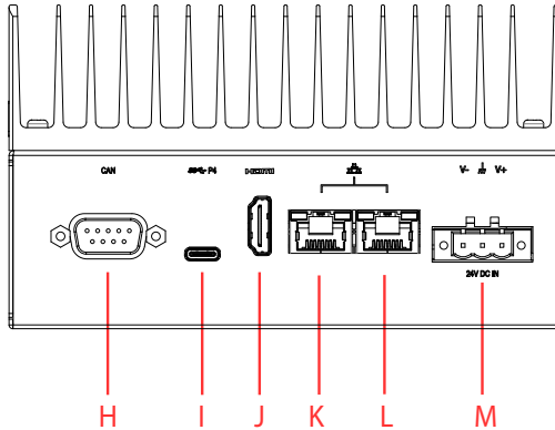
Figure 1-4: Side Panel I/O Connectors
