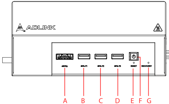
Figure 1-3: Front Panel I/O Connectors & Controls
